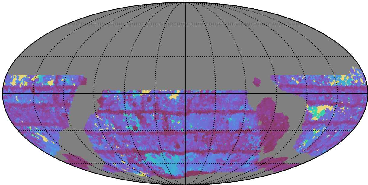
weather_cloudso6v3.4_10yrs WFD i band: Max Inter-Night Gap
