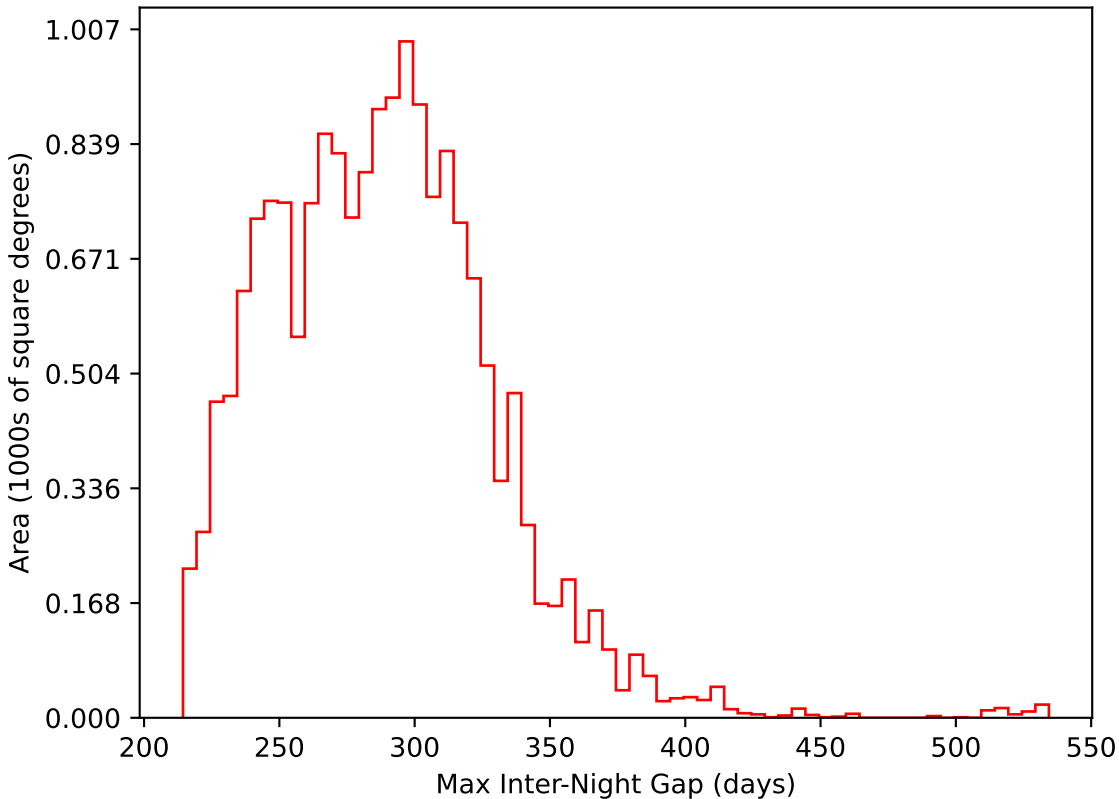
weather_cloudso6v3.4_10yrs WFD i band: Max Inter-Night Gap
