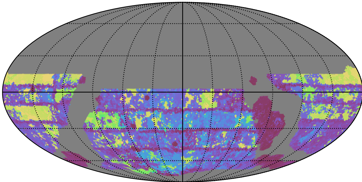
weather_cloudso6v3.4_10yrs WFD g band: Max Inter-Night Gap
