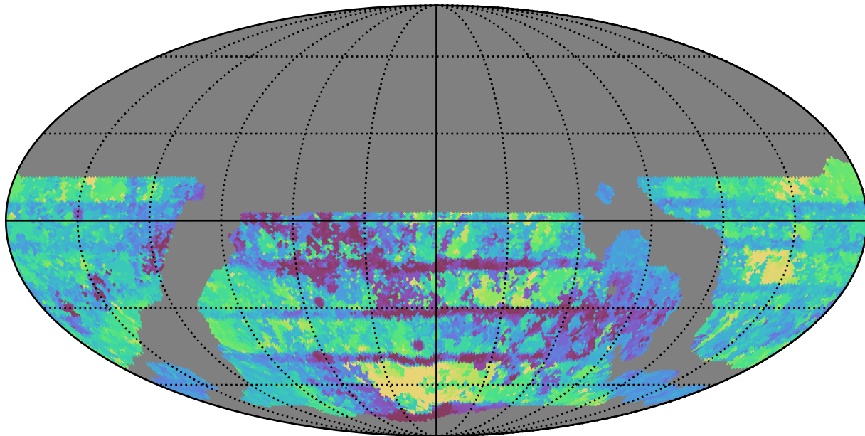
weather_cloudso6v3.4_10yrs WFD all bands: Max Inter-Night Gap
