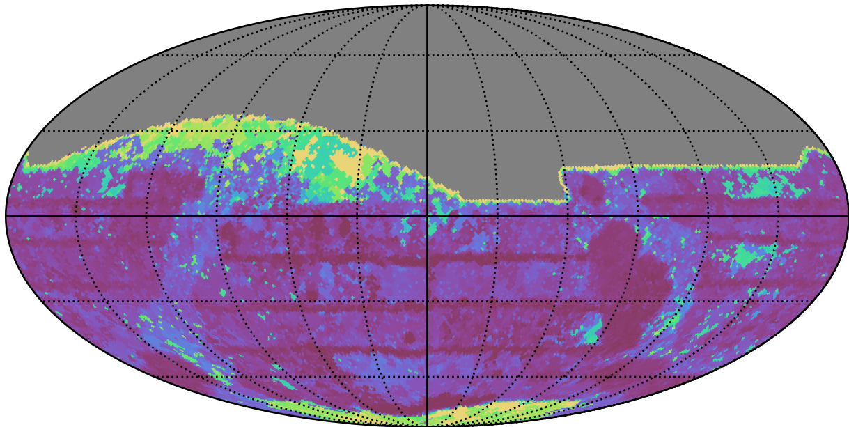
weather_cloudso6v3.4_10yrs All sky z band: Max Inter-Night Gap
