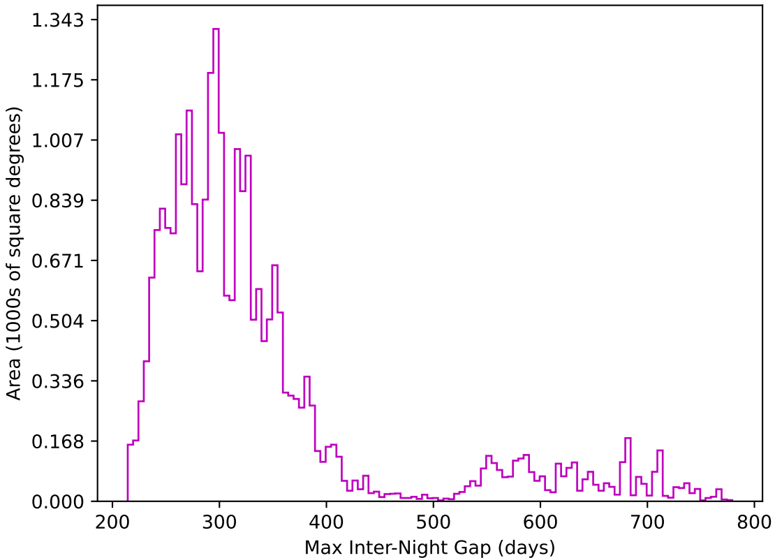
weather_cloudso6v3.4_10yrs All sky z band: Max Inter-Night Gap
