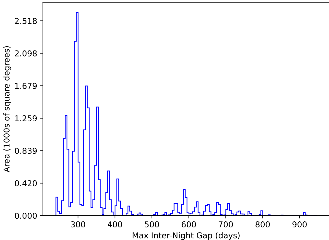
weather_cloudso6v3.4_10yrs All sky y band: Max Inter-Night Gap
