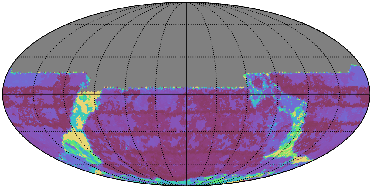
weather_cloudso6v3.4_10yrs All sky u band: Max Inter-Night Gap
