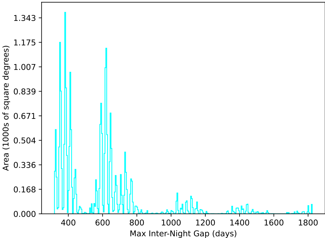
weather_cloudso6v3.4_10yrs All sky u band: Max Inter-Night Gap
