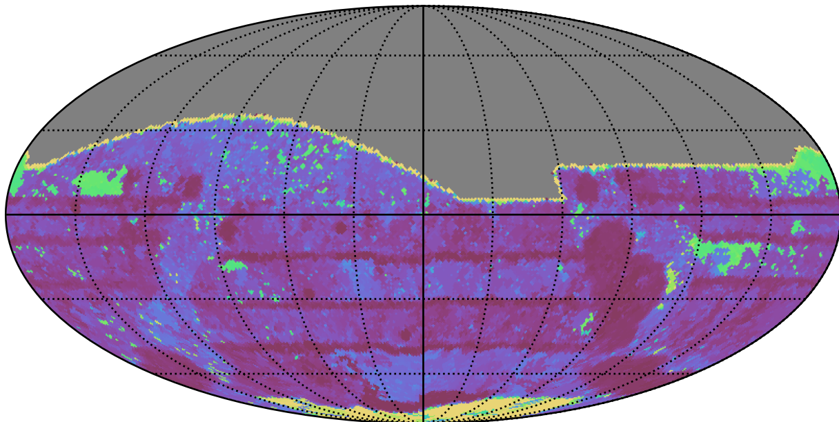
weather_cloudso6v3.4_10yrs All sky r band: Max Inter-Night Gap
