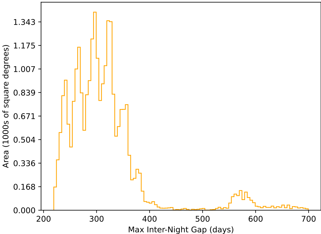
weather_cloudso6v3.4_10yrs All sky r band: Max Inter-Night Gap
