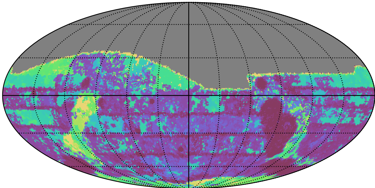
weather_cloudso6v3.4_10yrs All sky g band: Max Inter-Night Gap
