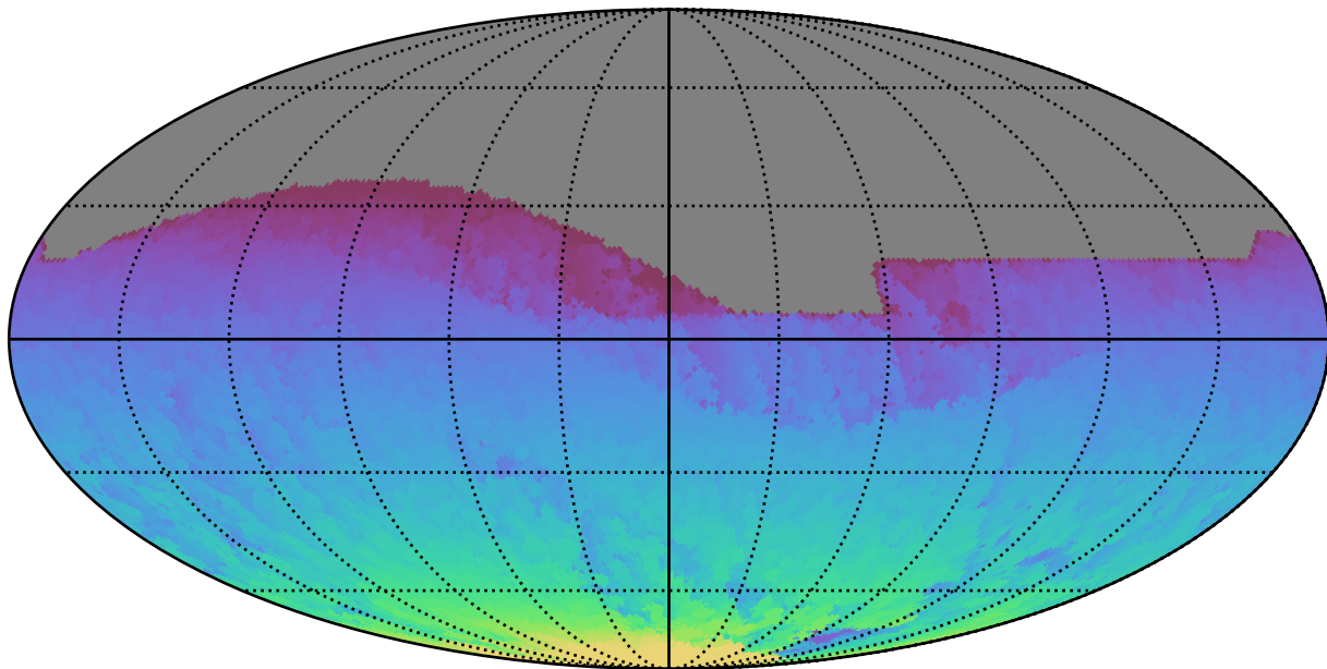
weather_cloudso6v3.4_10yrs All sky all bands: Max HA
