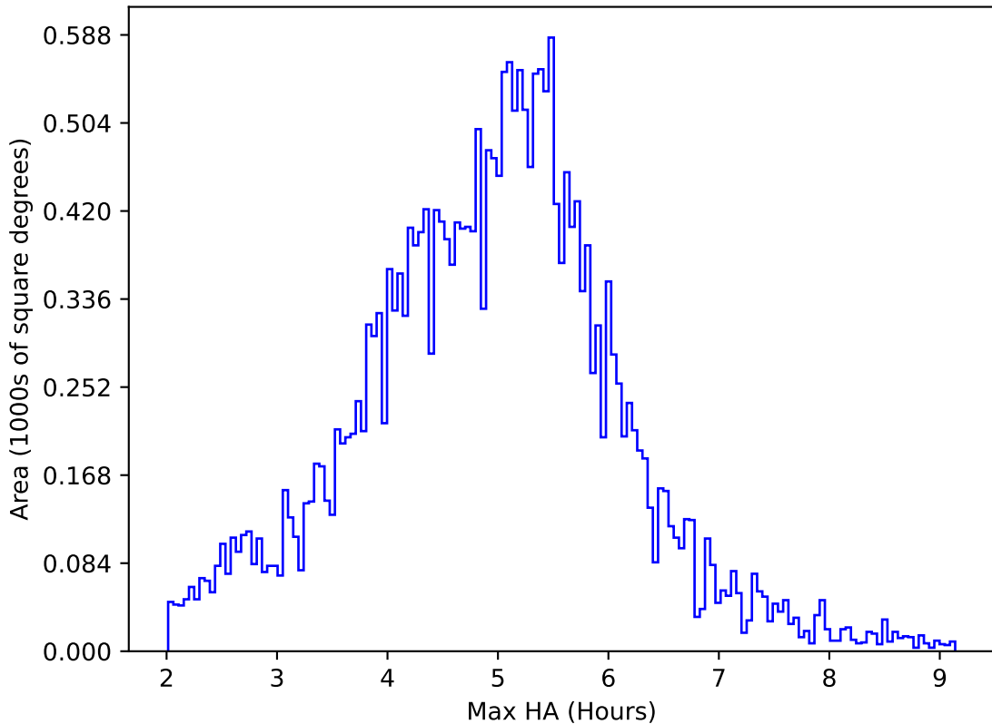
weather_cloudso6v3.4_10yrs All sky all bands: Max HA
