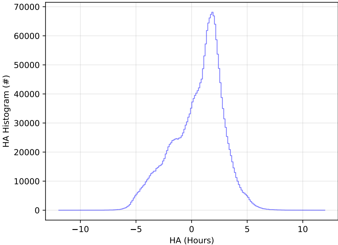
weather_cloudso6v3.4_10yrs All sky all bands: HA Histogram
