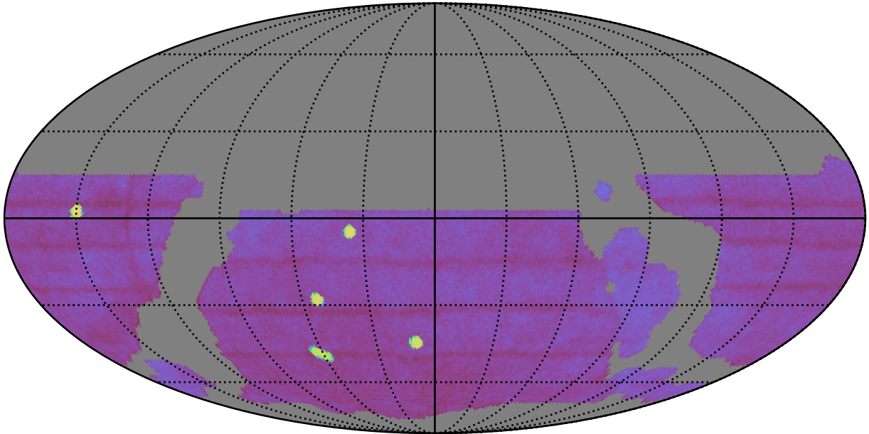
weather_cloudso6v3.4_10yrs gri WFD: Fraction of visits with a revisit < 60 min
