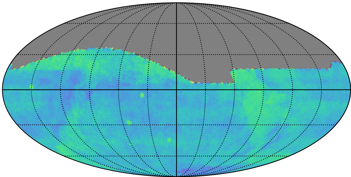
weather_cloudso6v3.4_10yrs gri All sky: Fraction of visits in pairs (20-90 min)
