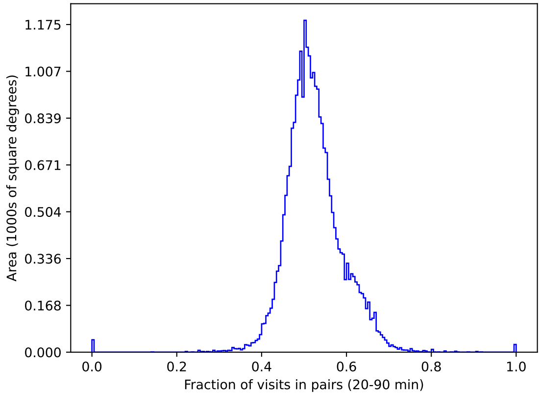
weather_cloudso6v3.4_10yrs gri All sky: Fraction of visits in pairs (20-90 min)
