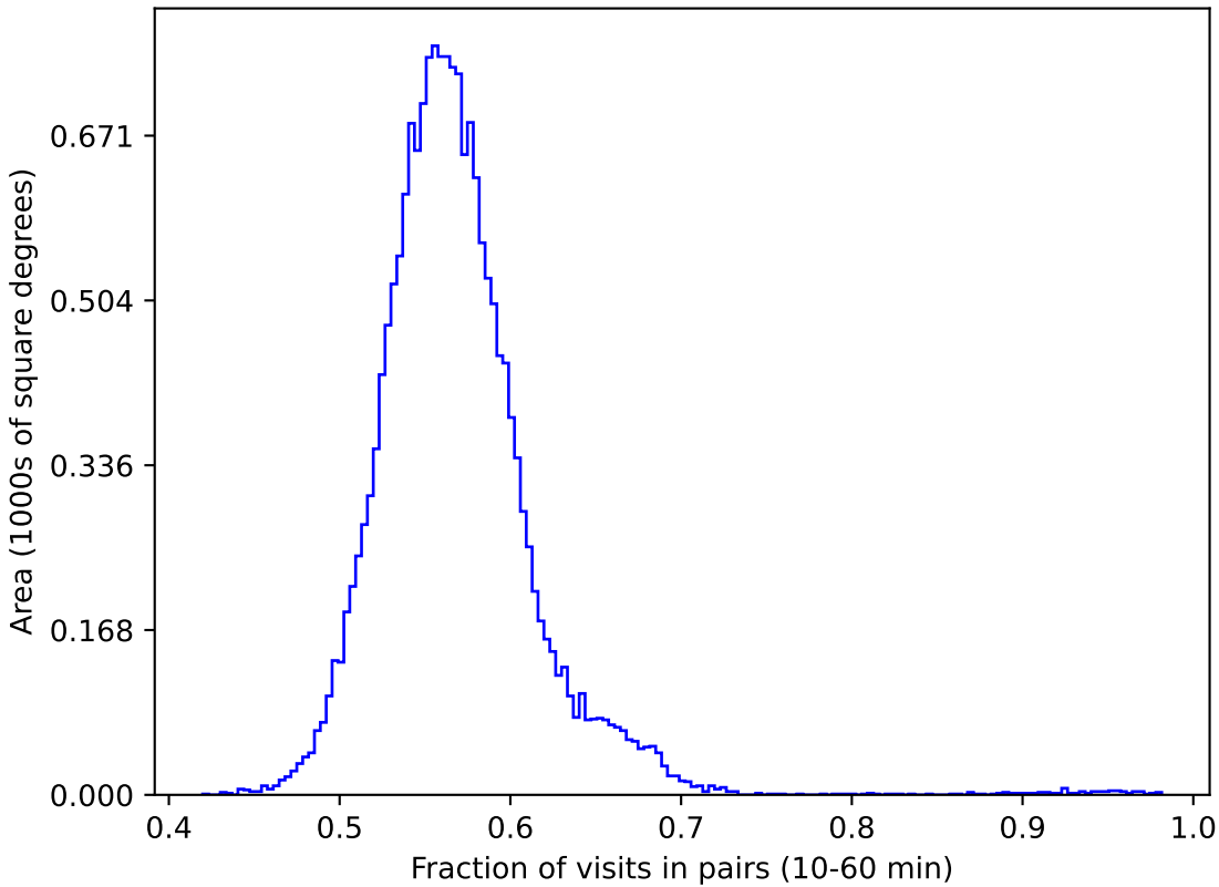
weather_cloudso6v3.4_10yrs gri WFD: Fraction of visits in pairs (10-60 min)
