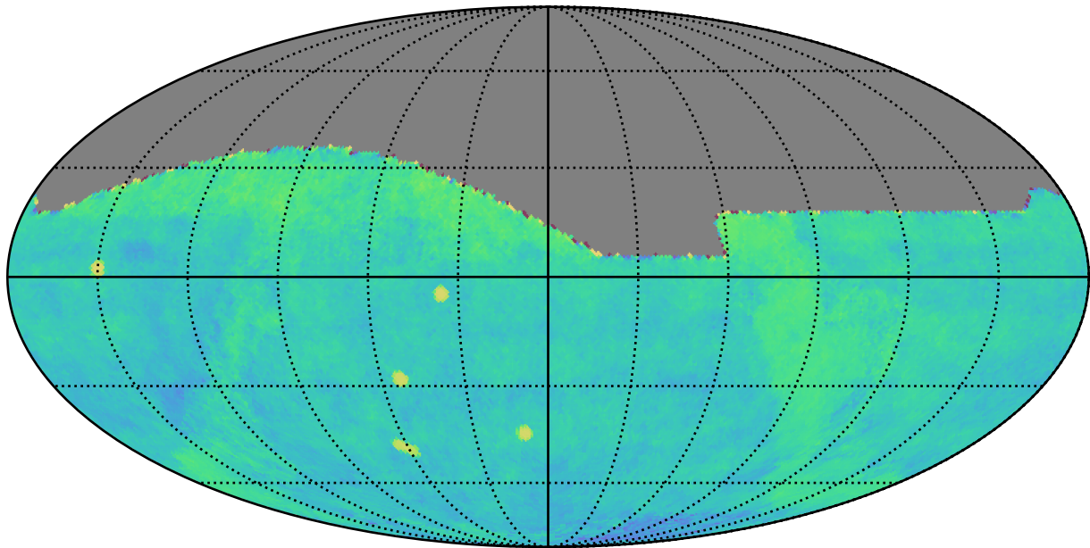
weather_cloudso6v3.4_10yrs gri All sky: Fraction of visits in pairs (10-60 min)
