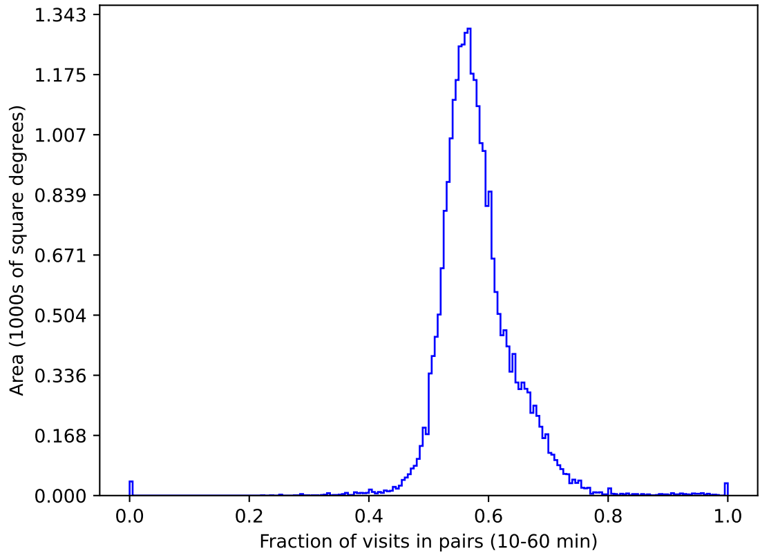
weather_cloudso6v3.4_10yrs gri All sky: Fraction of visits in pairs (10-60 min)
