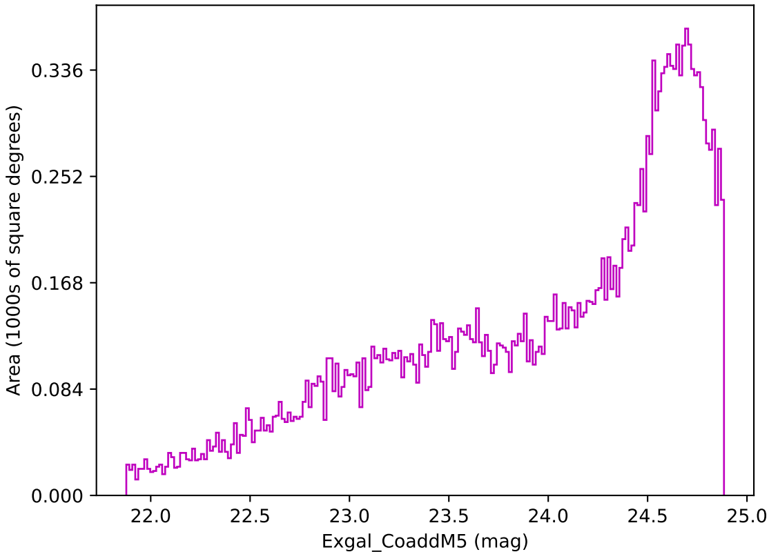
weather_cloudso6v3.4_10yrs Yr 3-4 z band: Exgal_CoaddM5
