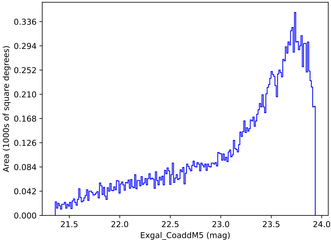
weather_cloudso6v3.4_10yrs Yr 3-4 y band: Exgal_CoaddM5
