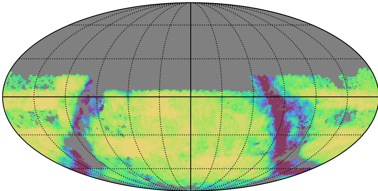
weather_cloudso6v3.4_10yrs Yr 3-4 u band: Exgal_CoaddM5
