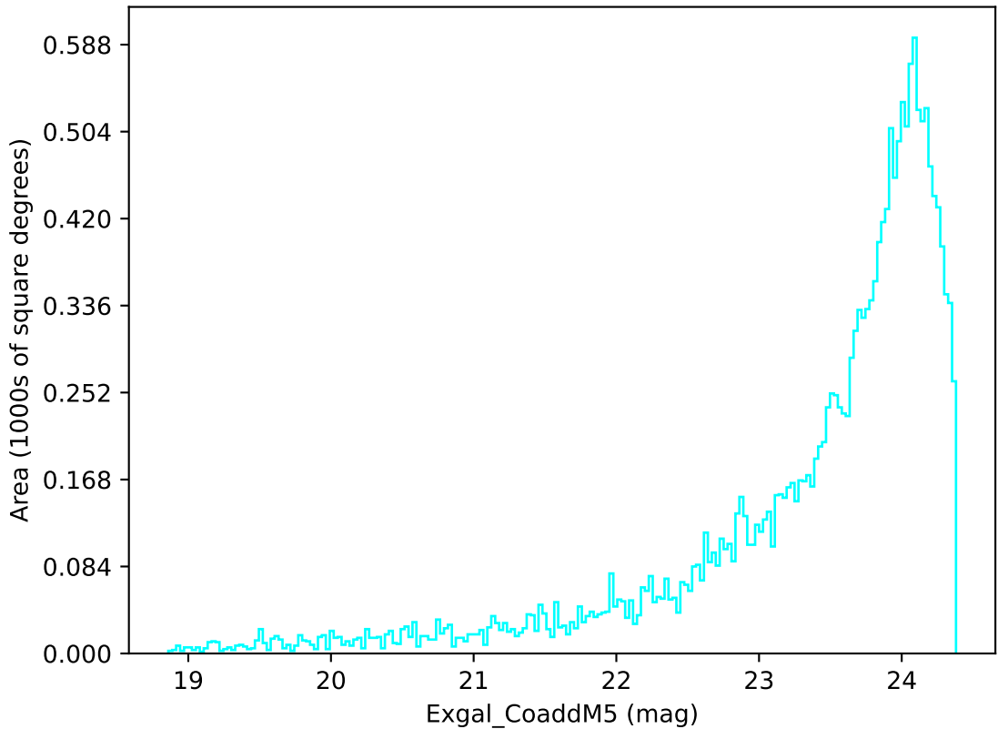
weather_cloudso6v3.4_10yrs Yr 3-4 u band: Exgal_CoaddM5
