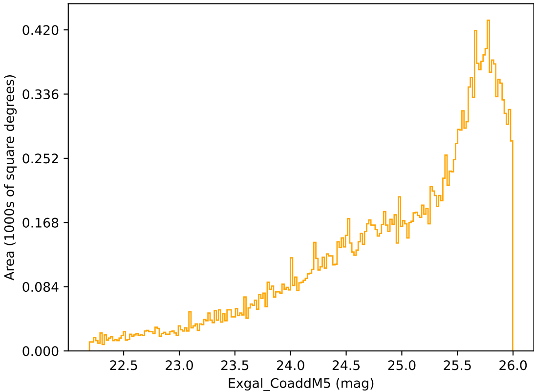
weather_cloudso6v3.4_10yrs Yr 3-4 r band: Exgal_CoaddM5
