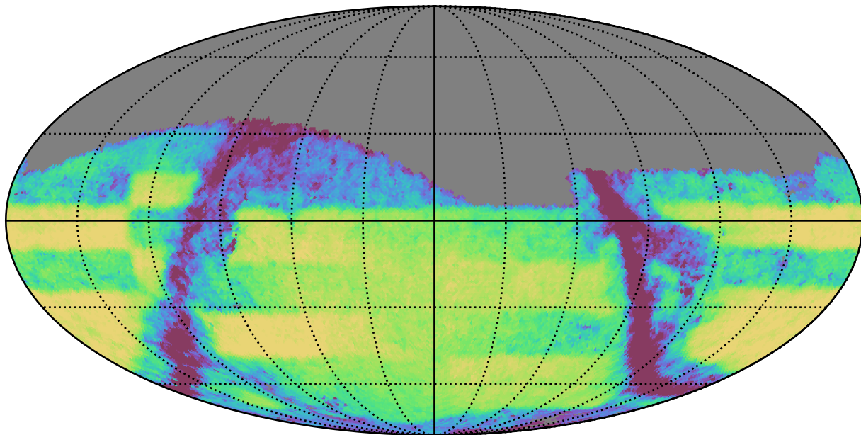
weather_cloudso6v3.4_10yrs Yr 3-4 i band: Exgal_CoaddM5
