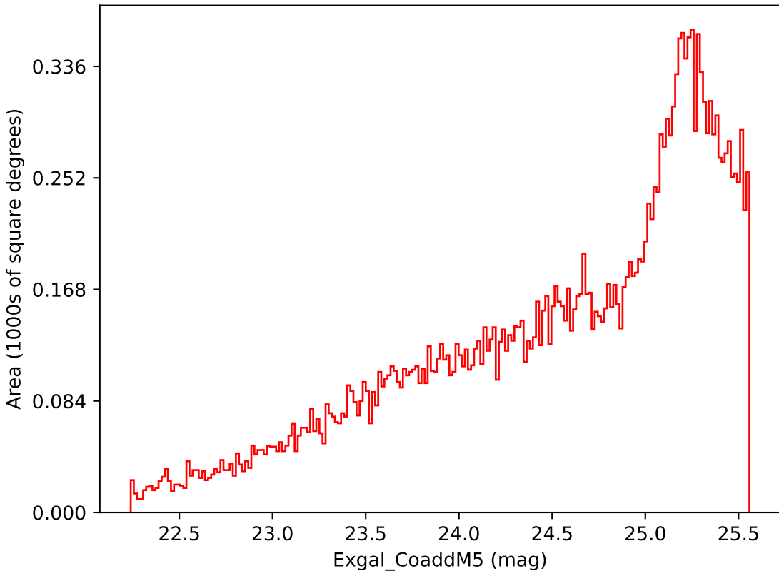
weather_cloudso6v3.4_10yrs Yr 3-4 i band: Exgal_CoaddM5
