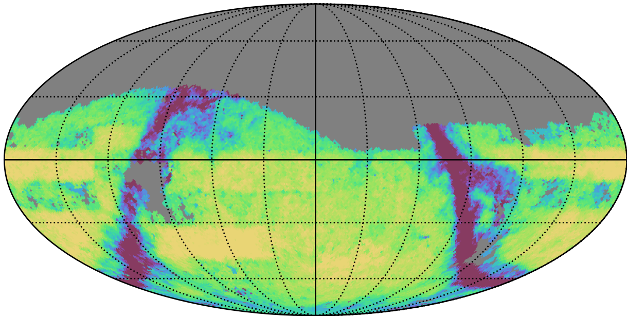
weather_cloudso6v3.4_10yrs Yr 3-4 g band: Exgal_CoaddM5
