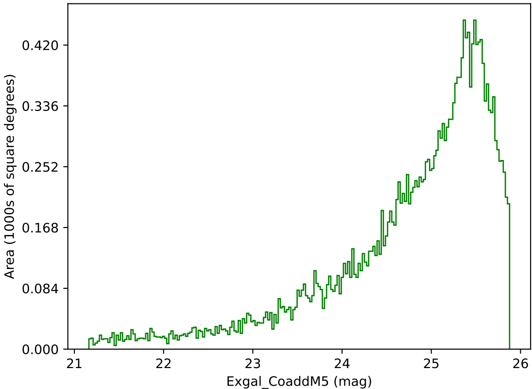
weather_cloudso6v3.4_10yrs Yr 3-4 g band: Exgal_CoaddM5
