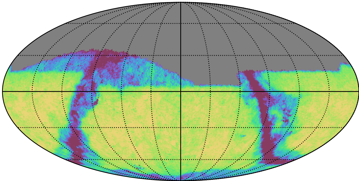
weather_cloudso6v3.4_10yrs Yr 1 z band: Exgal_CoaddM5
