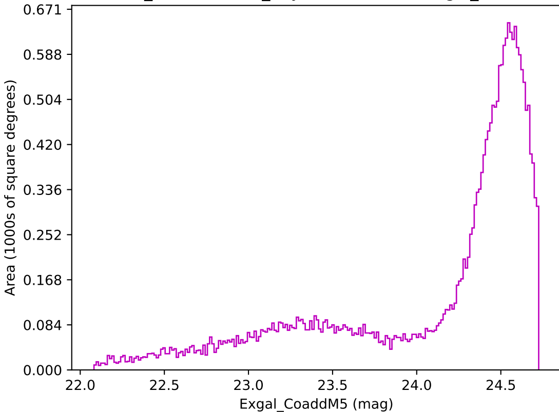
weather_cloudso6v3.4_10yrs Yr 1 z band: Exgal_CoaddM5
