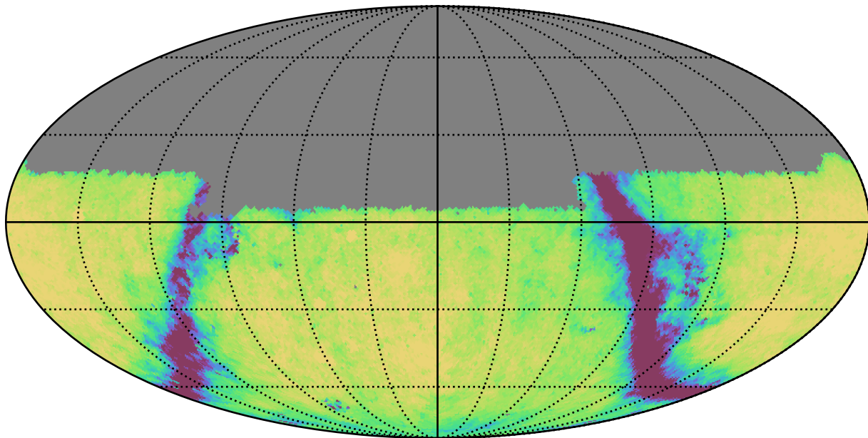
weather_cloudso6v3.4_10yrs Yr 1 u band: Exgal_CoaddM5
