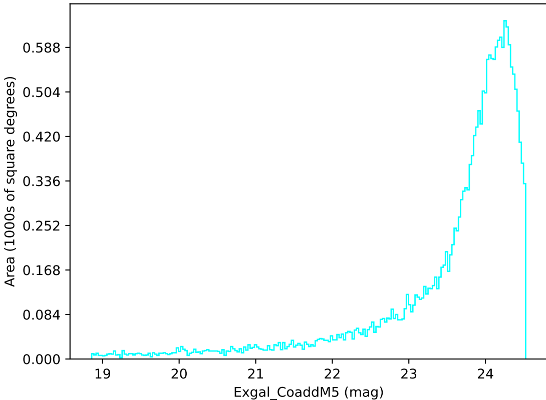
weather_cloudso6v3.4_10yrs Yr 1 u band: Exgal_CoaddM5
