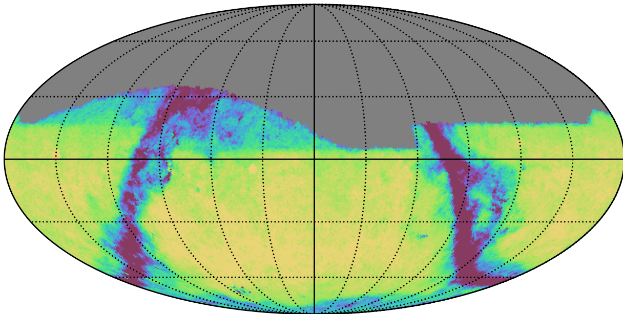
weather_cloudso6v3.4_10yrs Yr 1 r band: Exgal_CoaddM5
