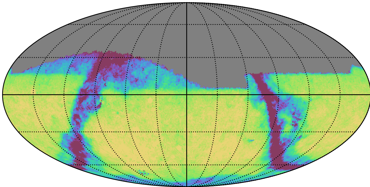
weather_cloudso6v3.4_10yrs Yr 1 i band: Exgal_CoaddM5
