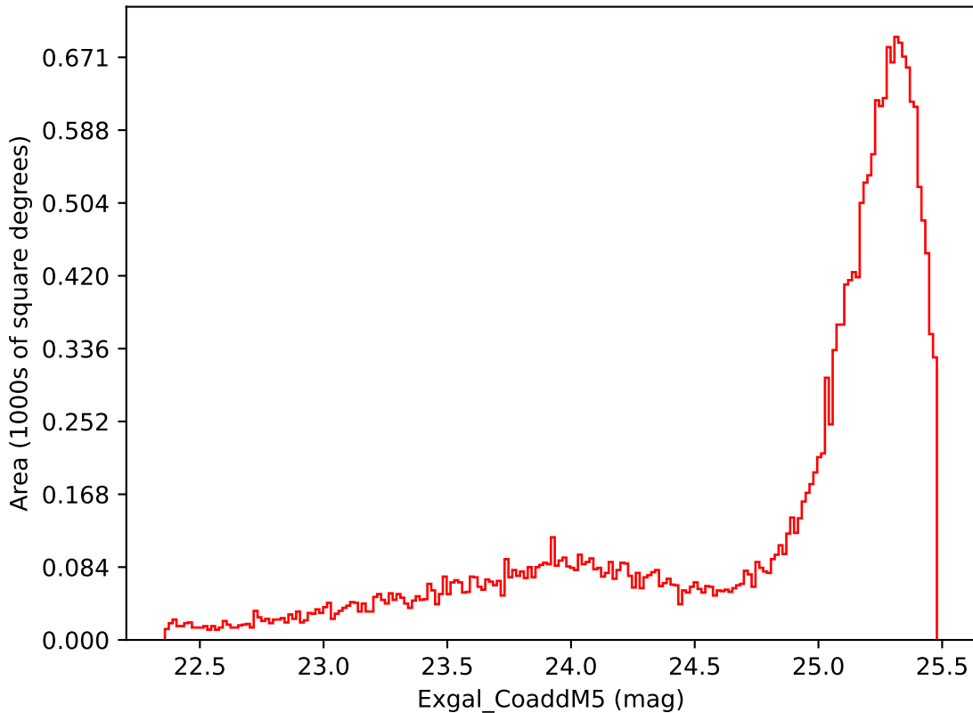
weather_cloudso6v3.4_10yrs Yr 1 i band: Exgal_CoaddM5
