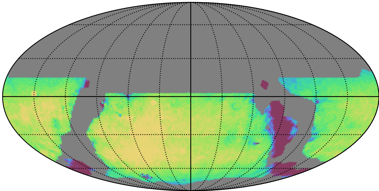
weather_cloudso6v3.4_10yrs WFD z band: Exgal_CoaddM5
