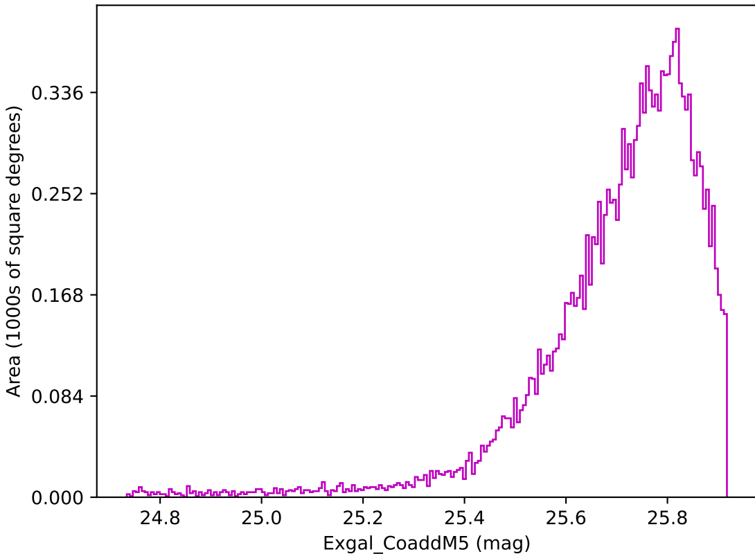
weather_cloudso6v3.4_10yrs WFD z band: Exgal_CoaddM5
