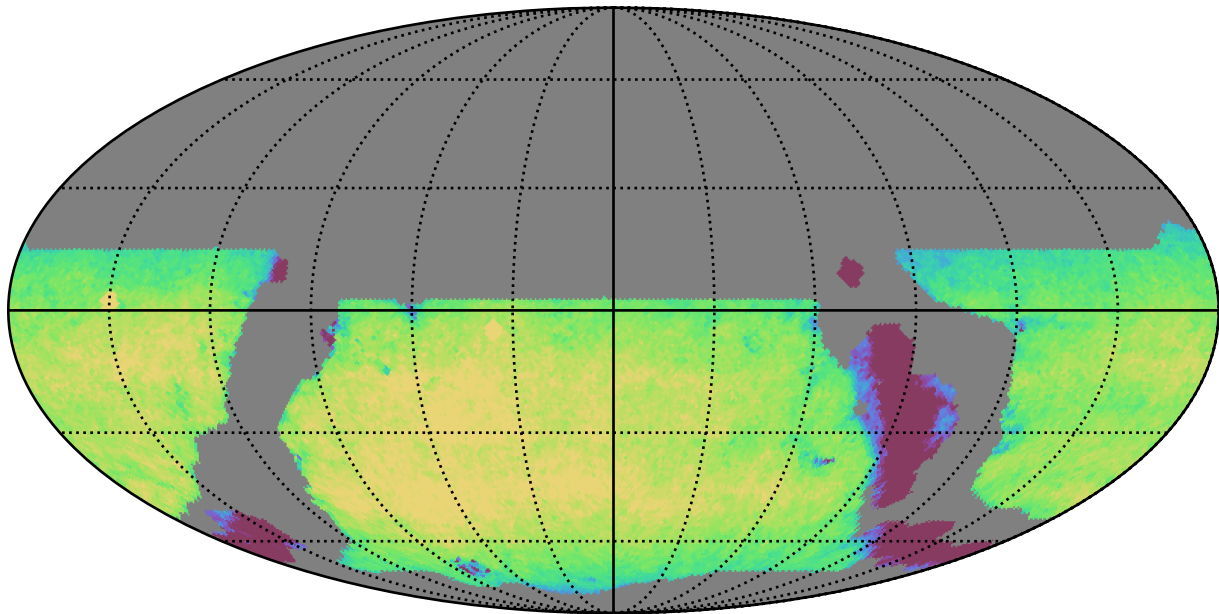
weather_cloudso6v3.4_10yrs WFD y band: Exgal_CoaddM5
