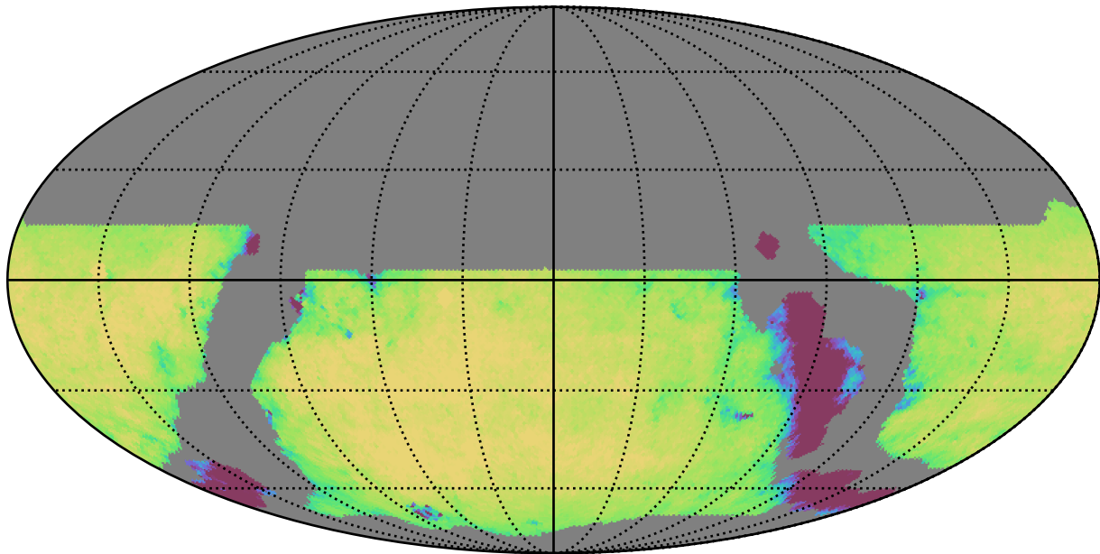
weather_cloudso6v3.4_10yrs WFD u band: Exgal_CoaddM5
