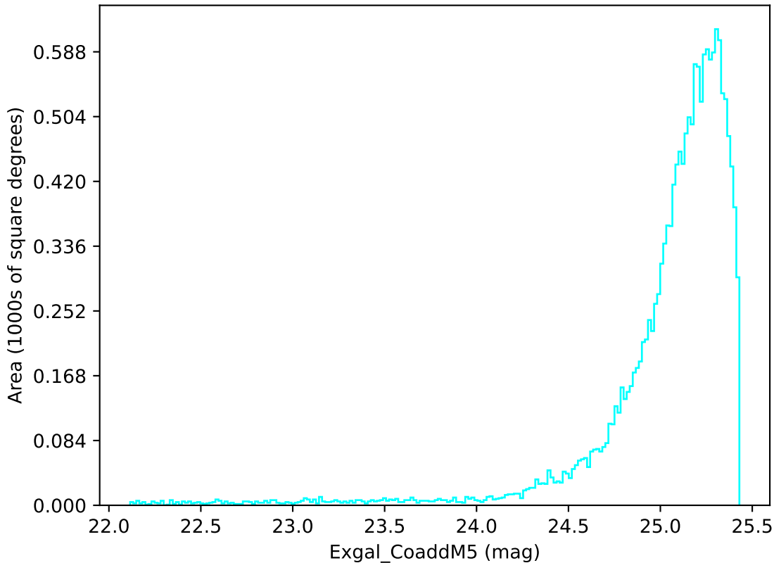
weather_cloudso6v3.4_10yrs WFD u band: Exgal_CoaddM5
