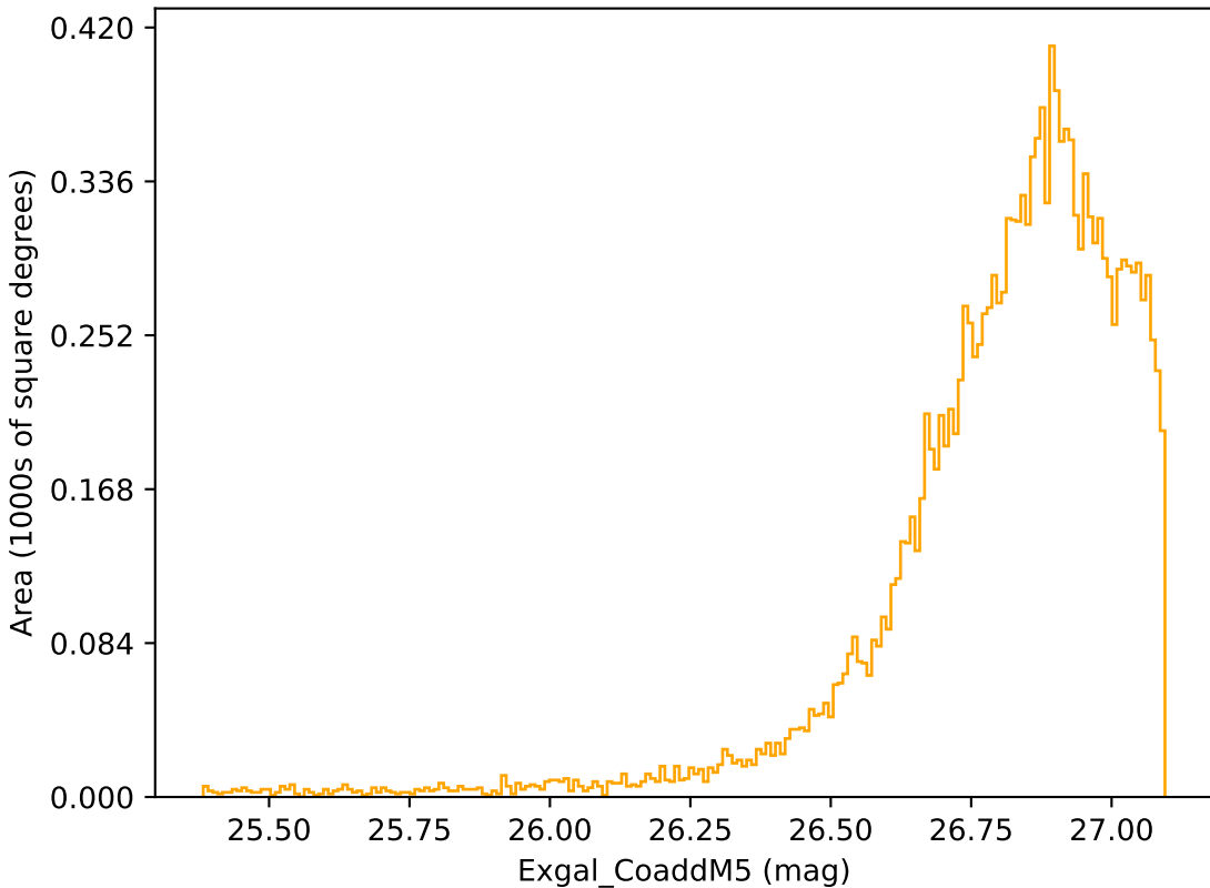
weather_cloudso6v3.4_10yrs WFD r band: Exgal_CoaddM5
