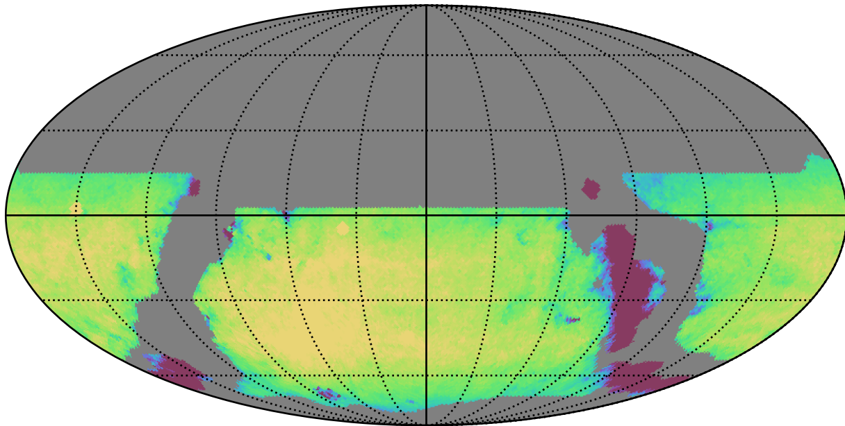
weather_cloudso6v3.4_10yrs WFD i band: Exgal_CoaddM5
