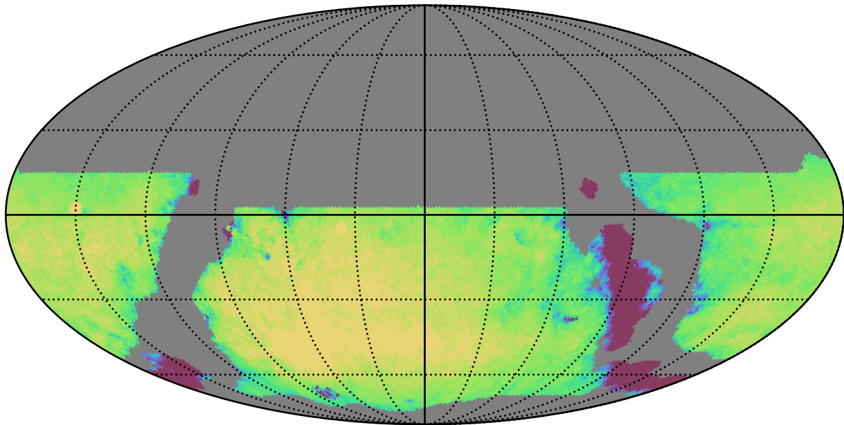
weather_cloudso6v3.4_10yrs WFD g band: Exgal_CoaddM5
