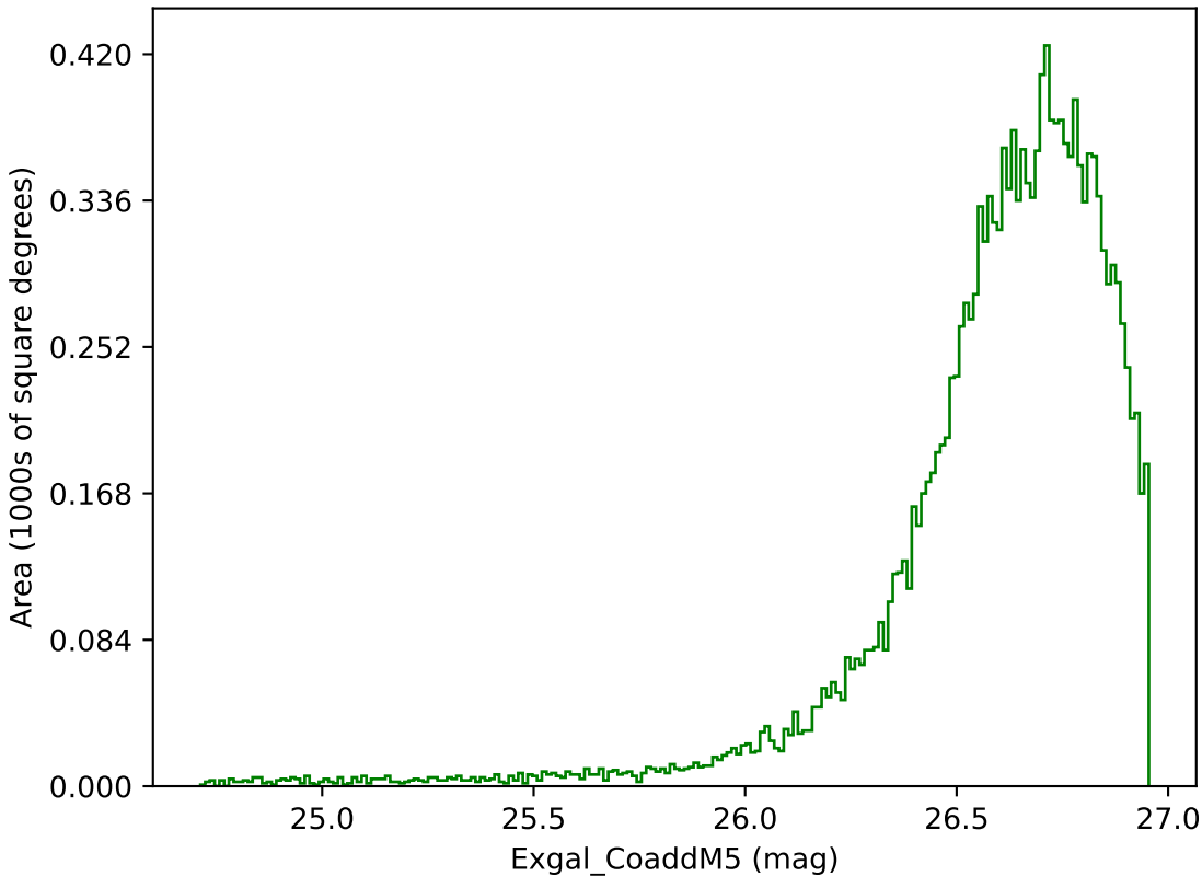
weather_cloudso6v3.4_10yrs WFD g band: Exgal_CoaddM5
