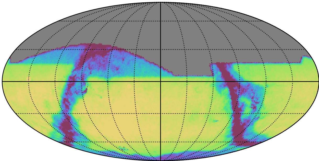
weather_cloudso6v3.4_10yrs All sky z band: Exgal_CoaddM5
