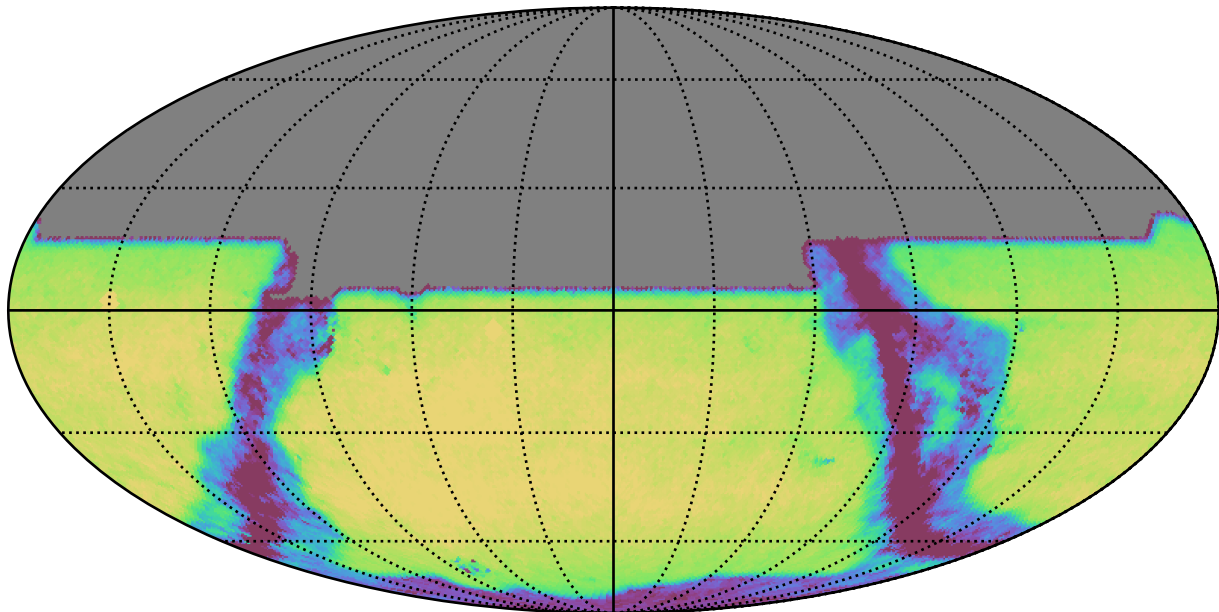
weather_cloudso6v3.4_10yrs All sky y band: Exgal_CoaddM5
