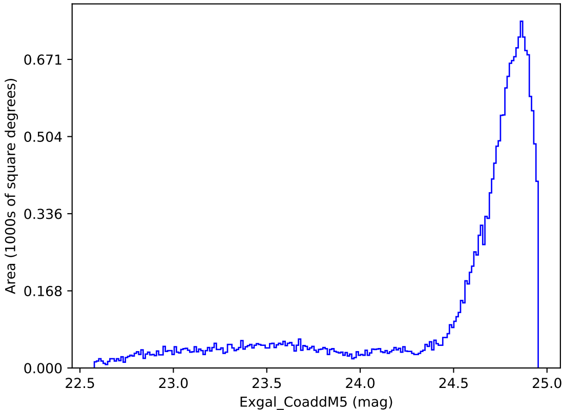
weather_cloudso6v3.4_10yrs All sky y band: Exgal_CoaddM5
