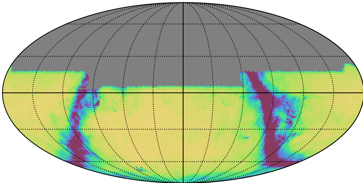
weather_cloudso6v3.4_10yrs All sky u band: Exgal_CoaddM5
